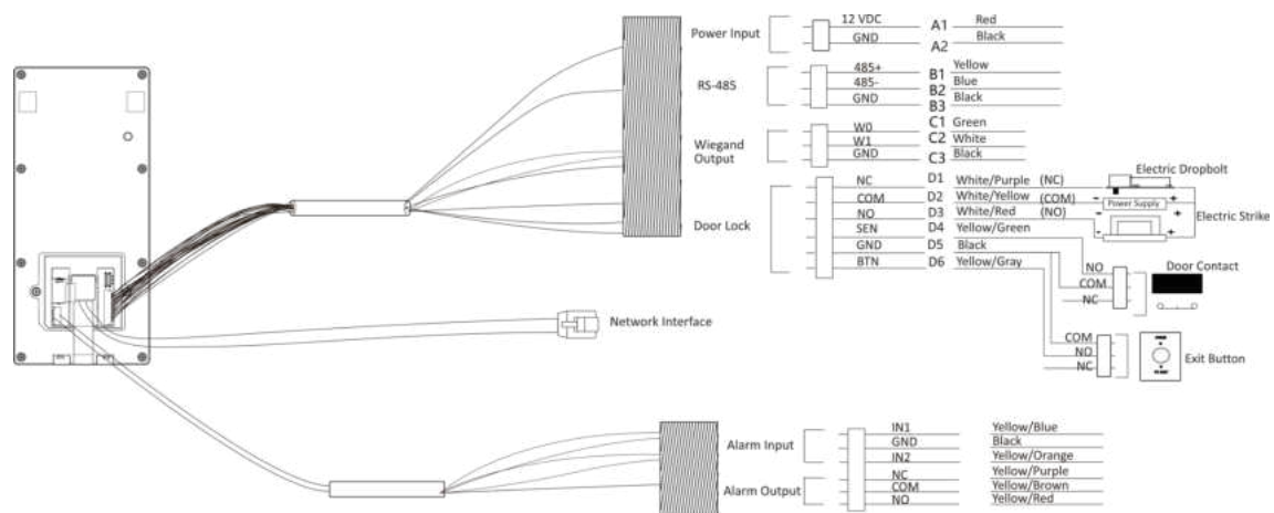
Figure 3-1 Terminal Diagram
