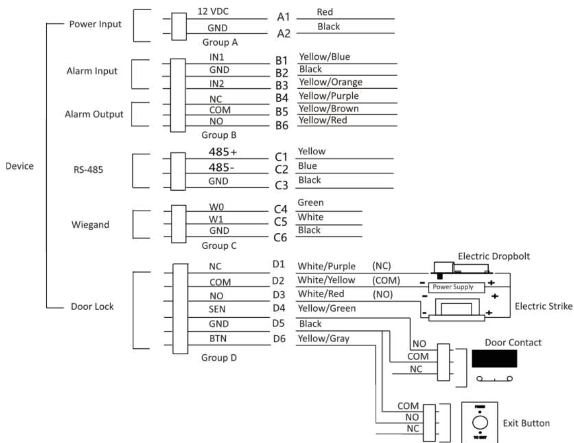
Figure 3-2 External Device Wiring
