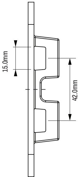
View on Side Face
