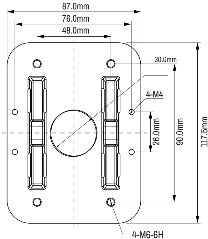
View on Front Face
