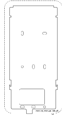
Drilling Template
