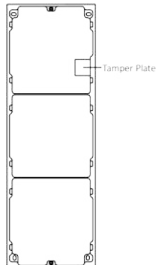
Figure 3-32 Mounting Frame
